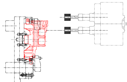
STATION 4 – DRILLING OF 5 MM DIAMETER HOLE
