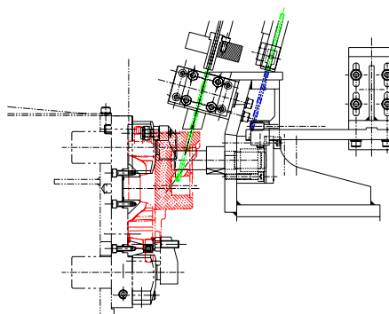
STATION 5 – DRILLING OF 4.1 MM DIAMETER HOLE
