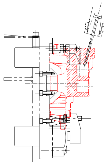
STATION 7 – TUBE DRIVE IN
