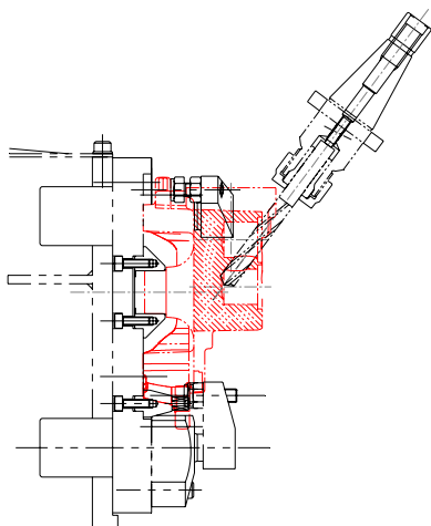
STATION 2 – DRILLING OF 10 MM DIAMETER HOLE
